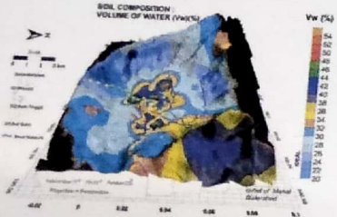
Fig. 6. Distribution of soil composition of the % water volume (Vw) combined with topography of Mahat watershed.
