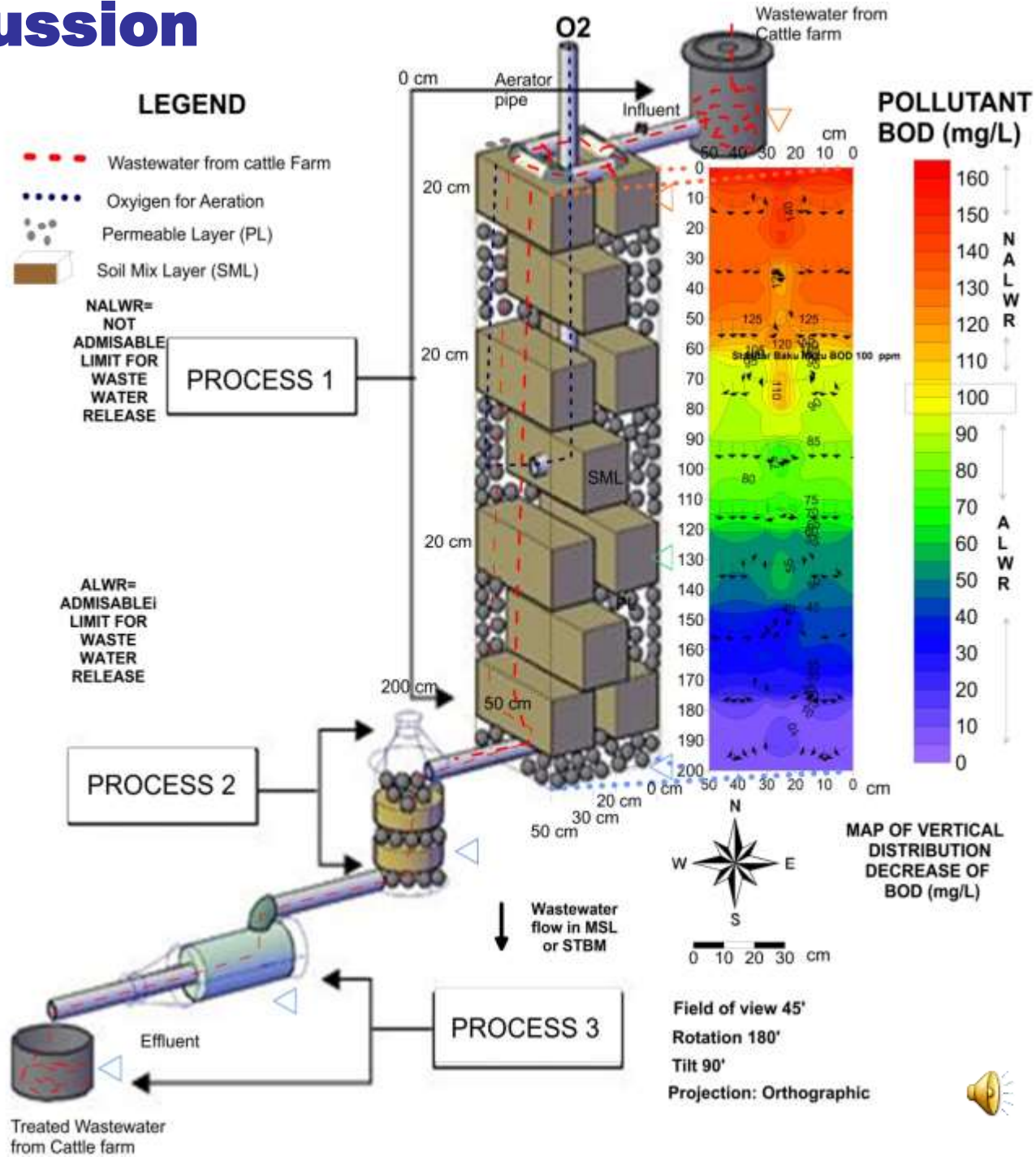
FIGURE 3. Vertical Distribution of Biological Oxygen Demand (BOD 5 ) in STBM system during purification of Cattle Farm wastewater
