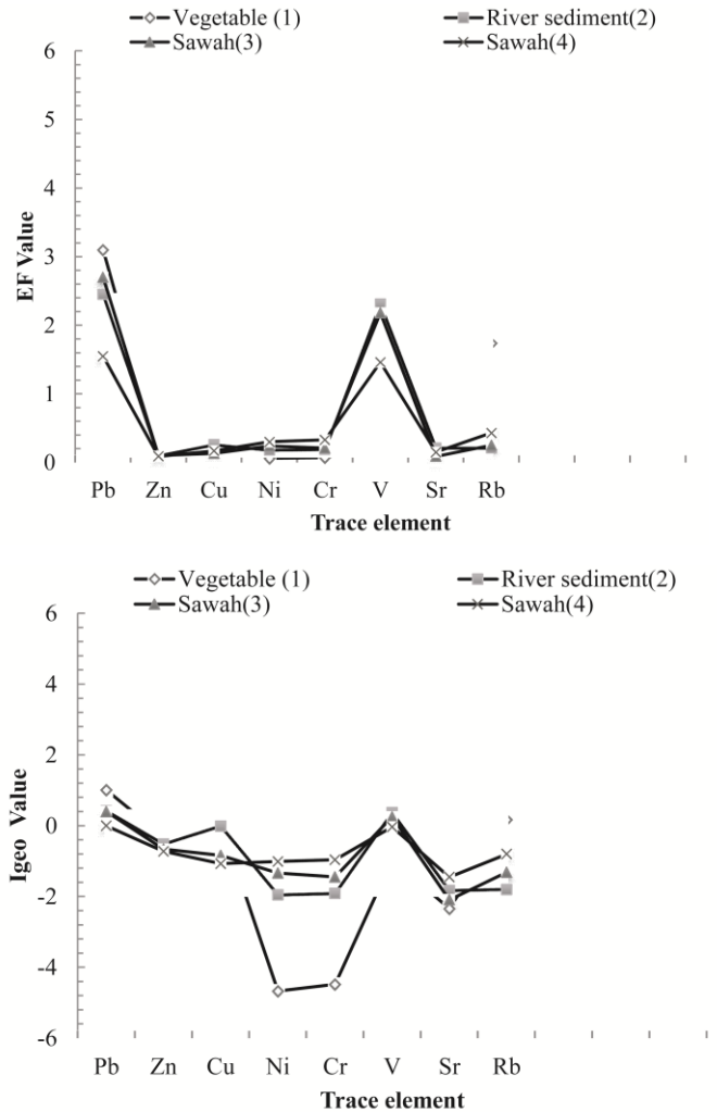
Figure 2. EF values and Igeo values in Vegetable, River sediment and sawah in Sumani watershed.
