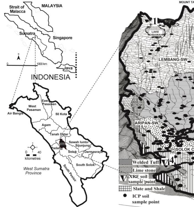
Figure 1. Study site, simplified basement geology and distribution of soil Sumatra, coordinates bases on UTM coordinate system WGS 84 Zone 47 S
