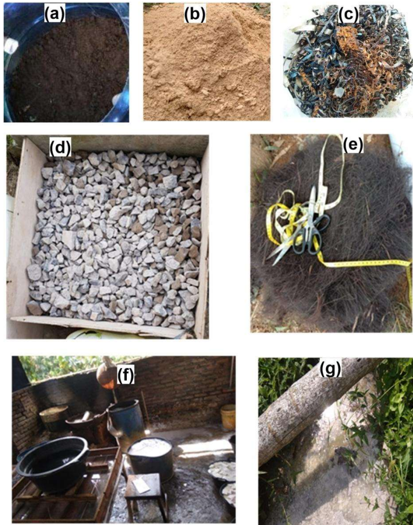
FIGURE 2. Materials for the MSL system and Tofu Factory Wastewater Sources: (a) Local soil, (b) sawdust, (c) iron lathe, (d) split stone, (e) Geotextile fibers, (f) Tofu Factory and (g) disposal of tofu factory wastewater.
