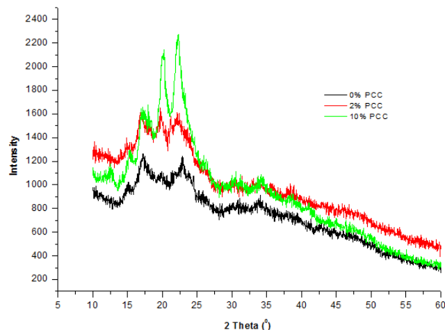
Fig. 4 XRD spectra of bioplastic/PCC composites
