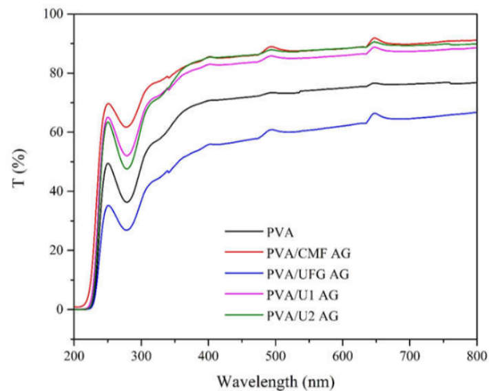
Fig. 4. Transmittance versus wavelength of all samples.
