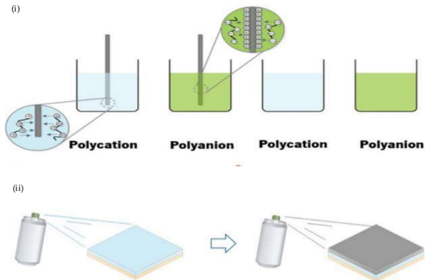
Figure 6. (i) Dipping and (ii) spray coating method [16].
