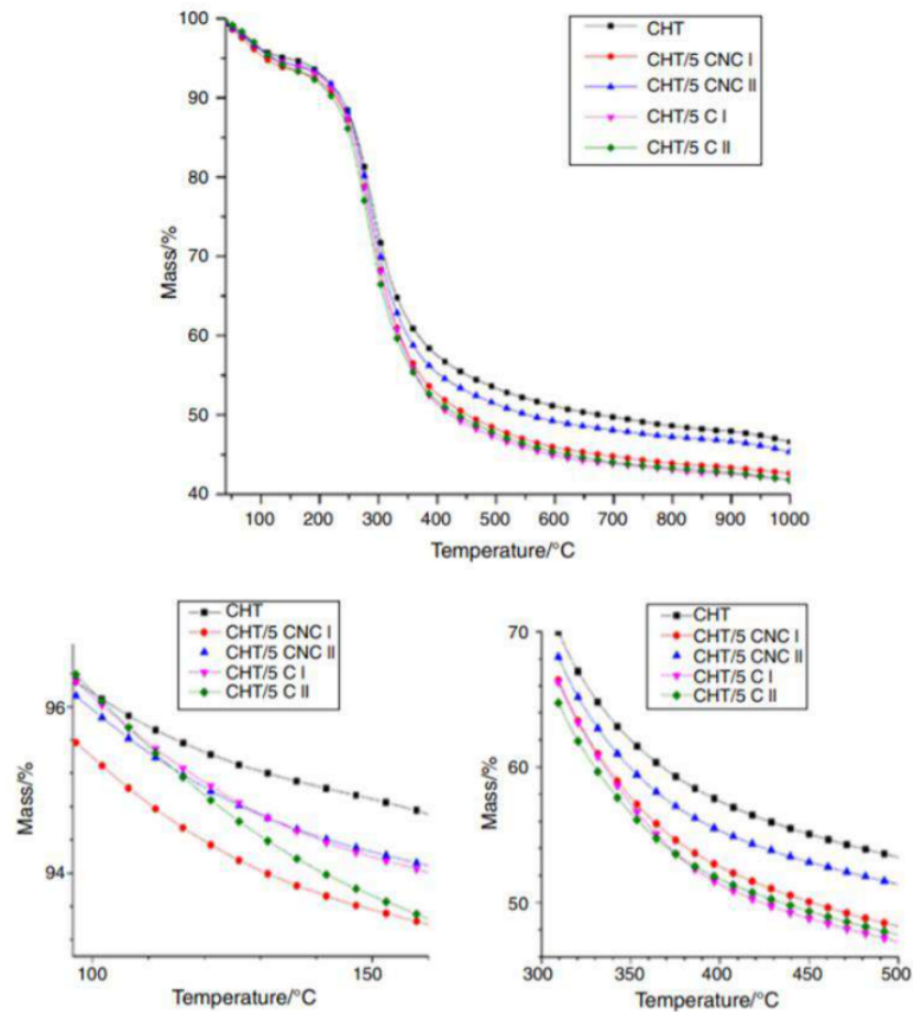
Figure 10. Thermogravimetric curves for chitosan and its composites [91].
