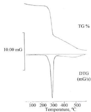
Figure 4. Thermogravimetric curves for chitosan [95]. (Mostafa Amin, 2012).
