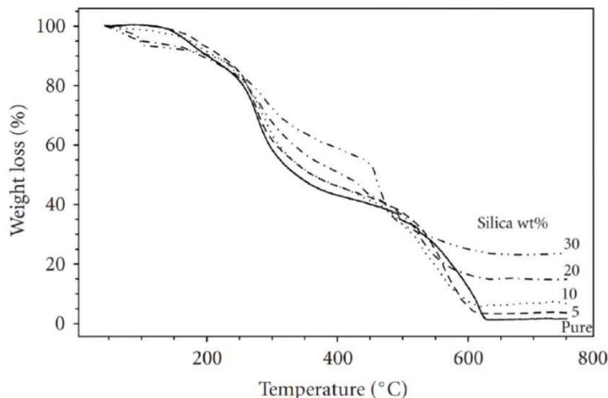
Figure 12. Thermogravimetric curves for chitosan-Si nanocomposites [156].
