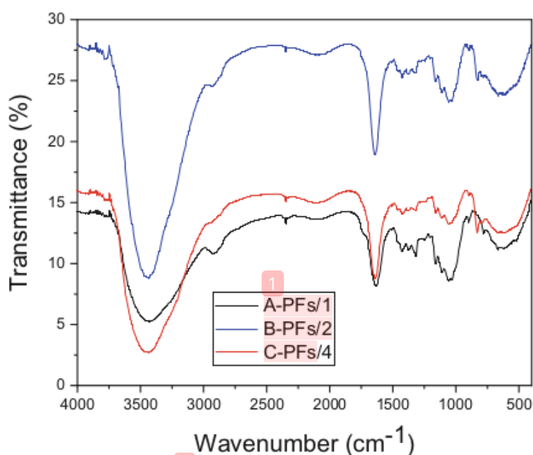
Fig. 2. FTIR of A-PFs/1, B-PFs/2, and C-PFs/4 samples
