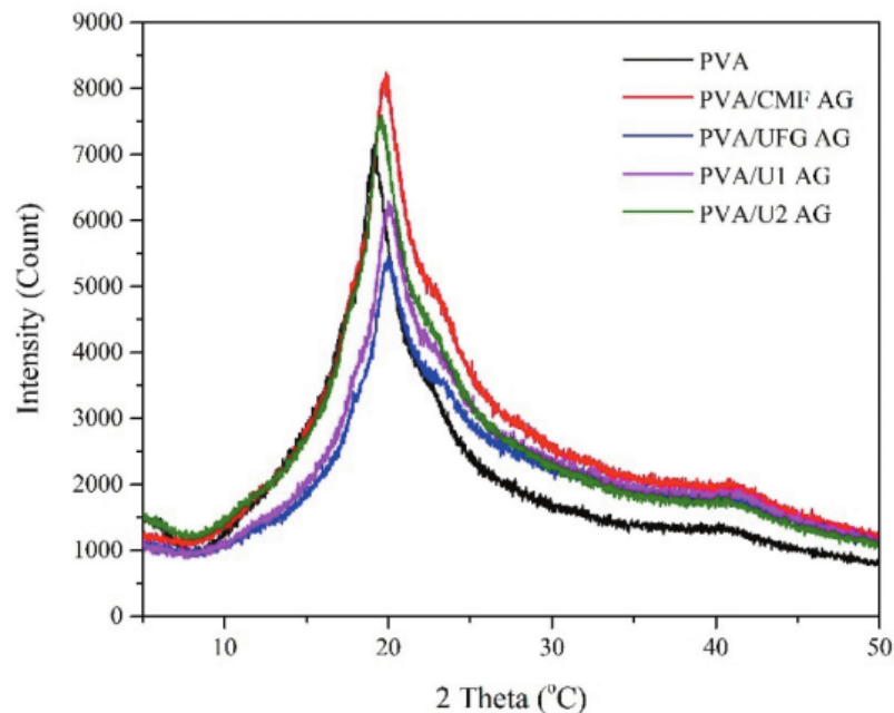
Figure 5. The XRD patterns of all samples.
