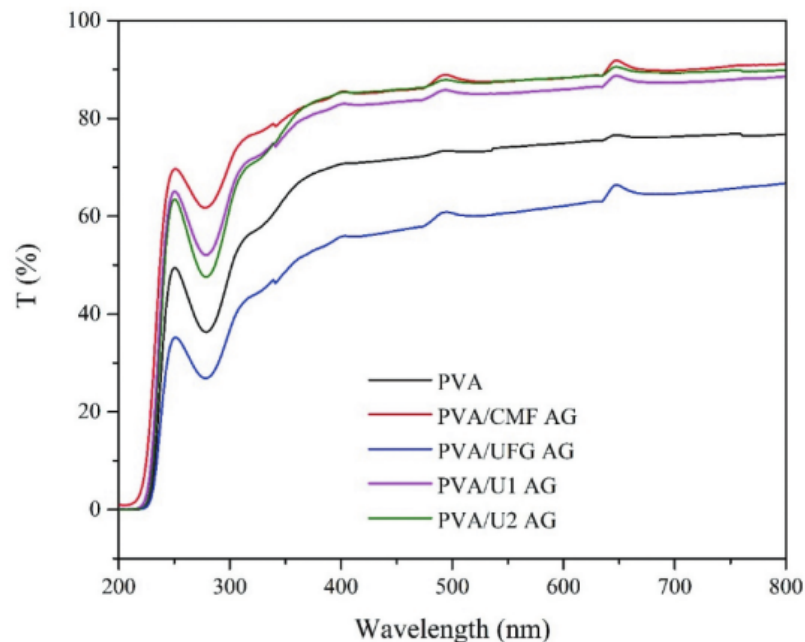
Figure 3. Transmittance versus wavelength of all samples.
