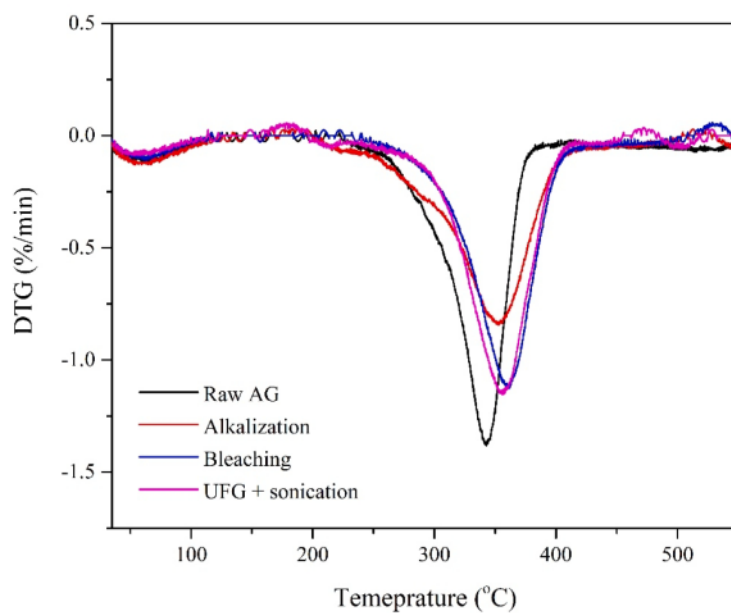
Fig. 5. TGA curve (a), DTG curve (b) of raw fibers, alkalized, bleaching, and mechanical treatment.
